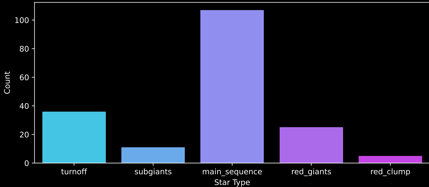
APOGEE DR17 Field: [157+60_MGA] Count plot of Star Type
