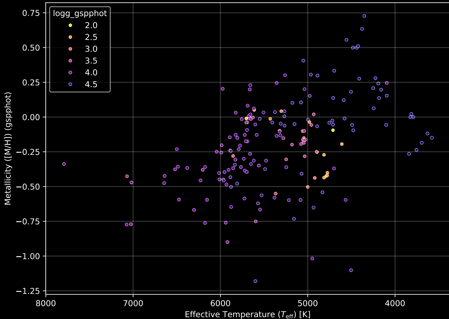
APOGEE DR17 Field: [157+60_MGA] Stellar Population Parameters (n= 184)
