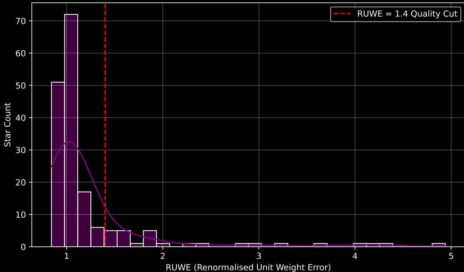
GAPOGEE DR17 Field [157+60_MGA] RUWE Distribution (n= 173)
