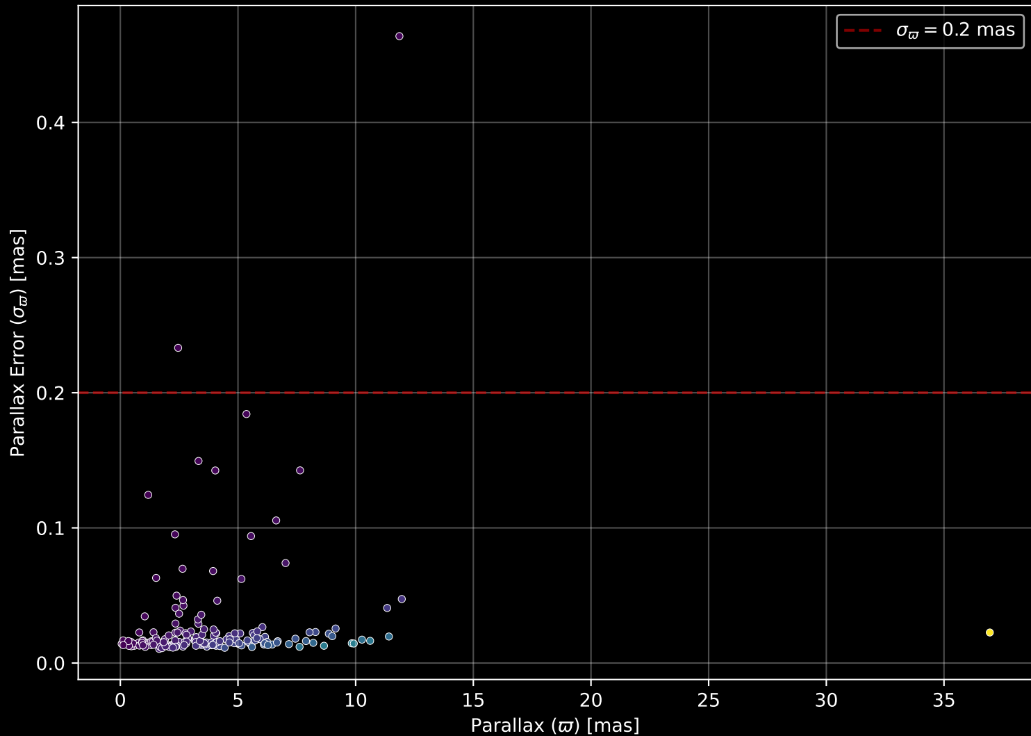
APOGEE DR17 Field: [157+60_MGA] Parallax Quality (n= 184)
