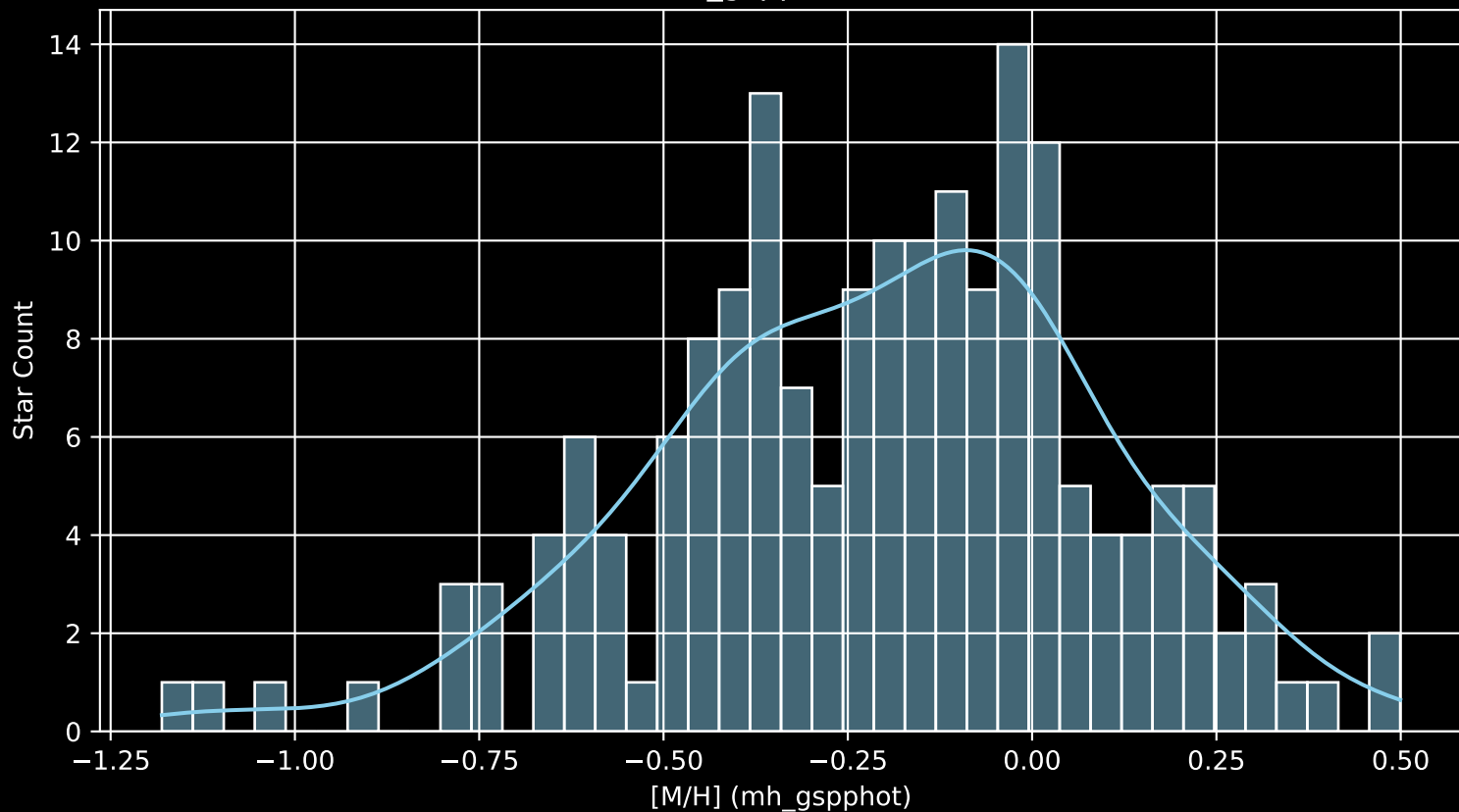
APOGEE DR17 Field: [157+60_MGA [M/H] (mh_gspphot) (n= 180)
