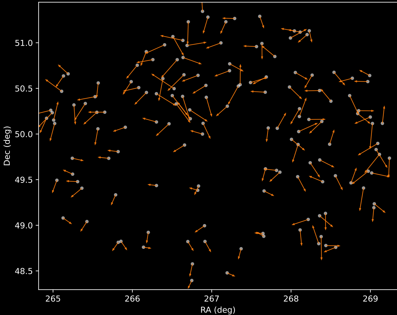
APOGEE DR17 Cluster 2 Proper Motion Vectors (n=146)
