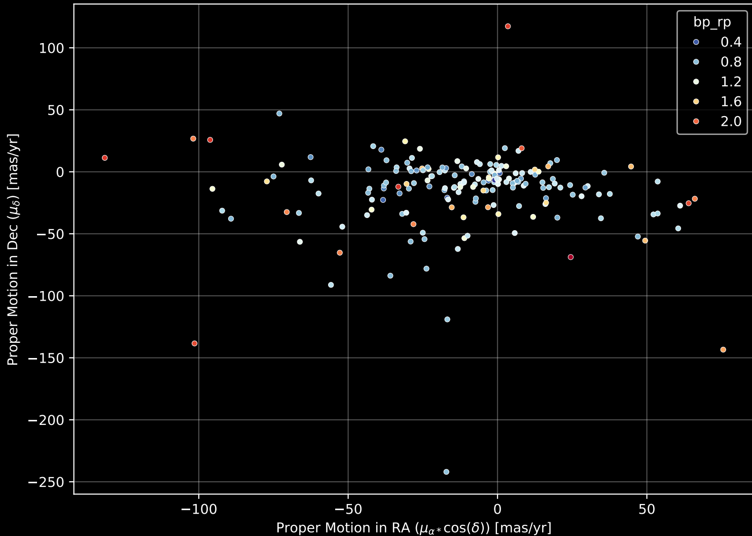
APOGEE DR17 Field: [157+60_MGA] Proper Motion Diagram (n= 184)
